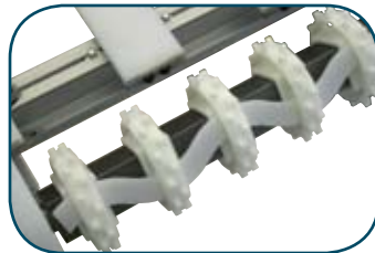
Patented Sprocket Alignment Key provides quick belt alignment
